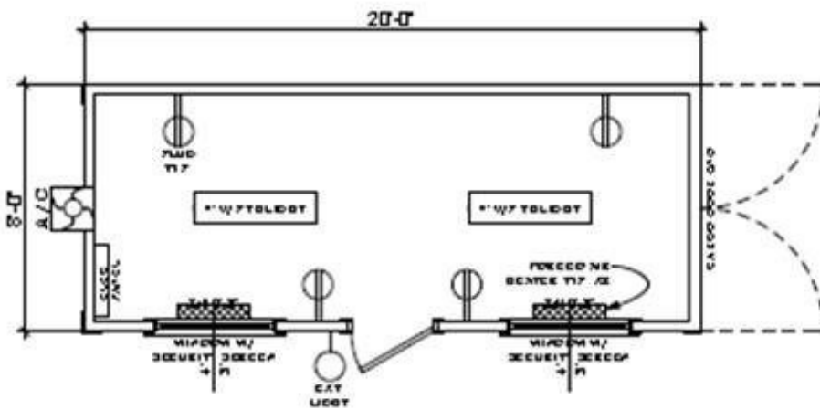
8' X 20' CONTAINER OFFICE PLAN VIEW SCALE 1/2" = 1'-0"
