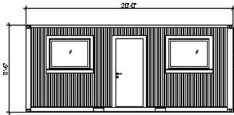
ELEVATION SCALE 1/2" = 1'-0"
