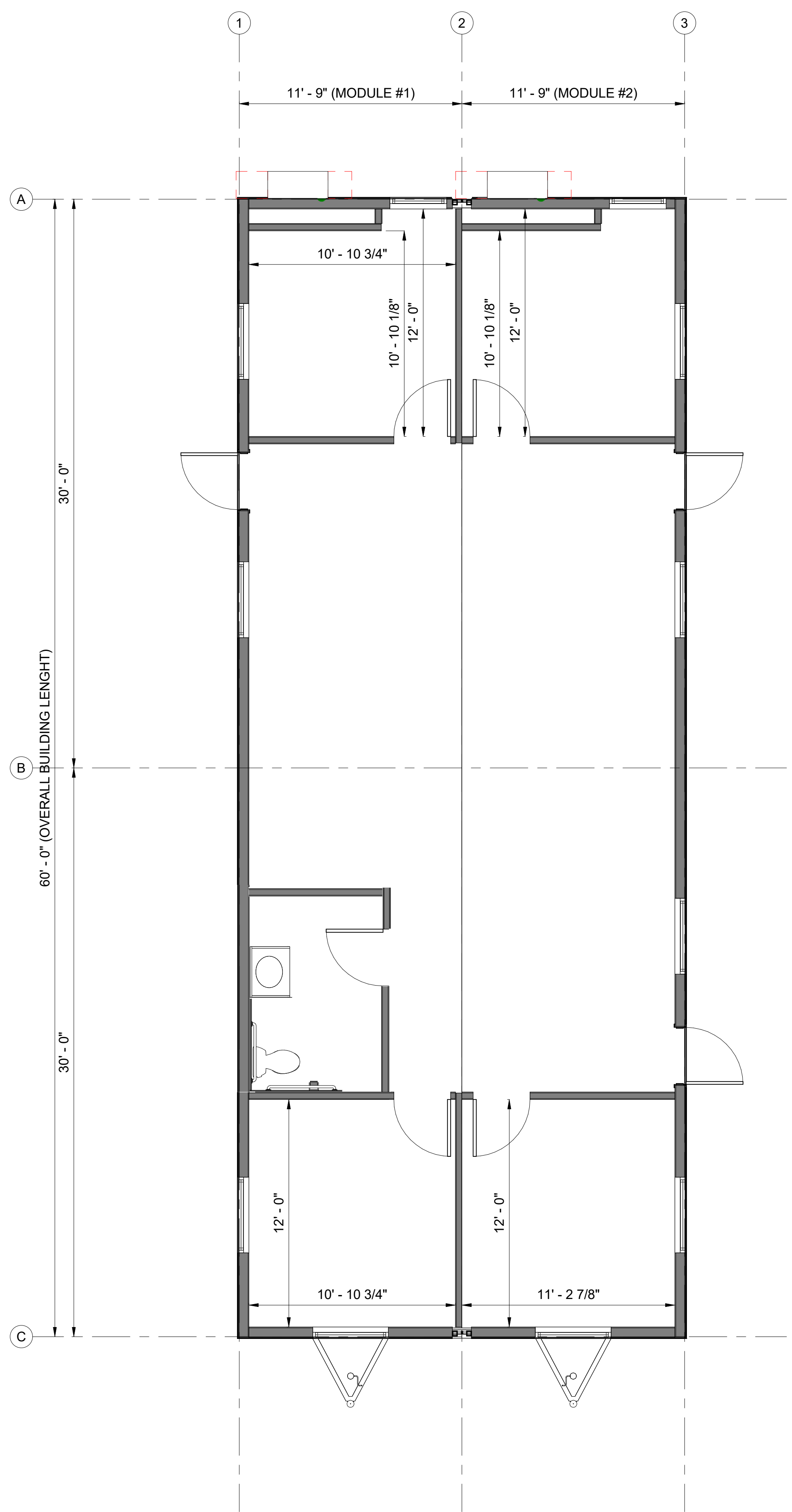
1 OVERALL FLOOR PLAN 1/4" = 1'-0"
