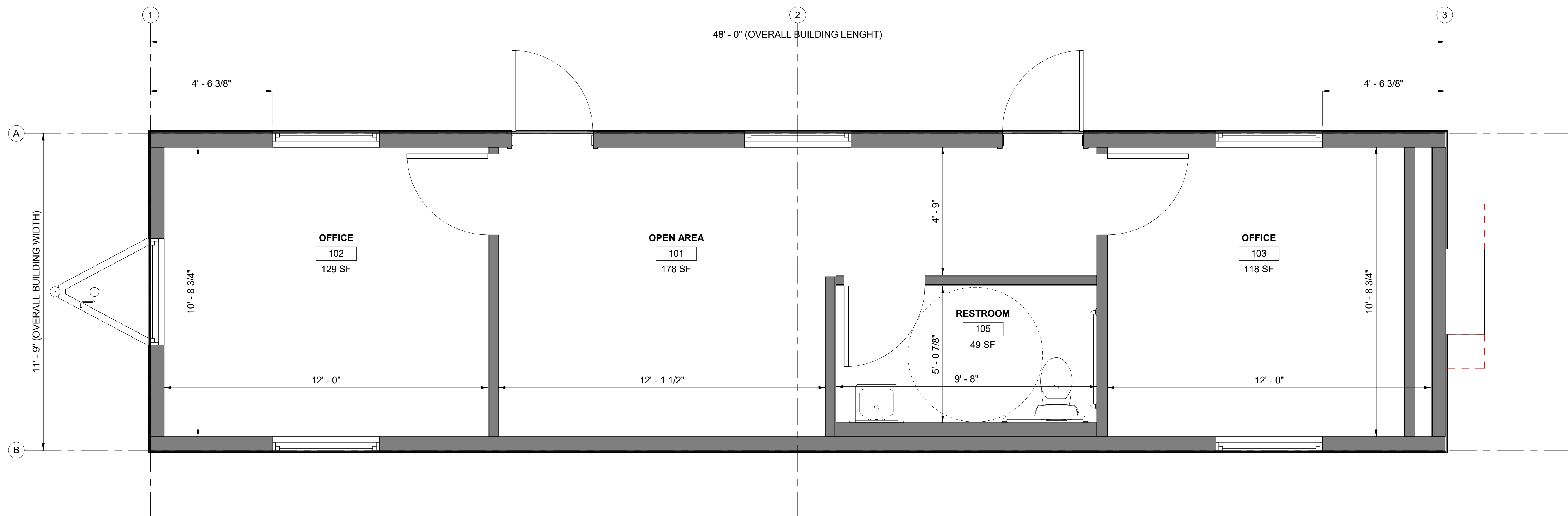
1 ARCHITECTURAL FLOOR PLAN 1/2" = 1'-0"
